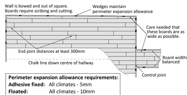
Figure 3 – Scribing
