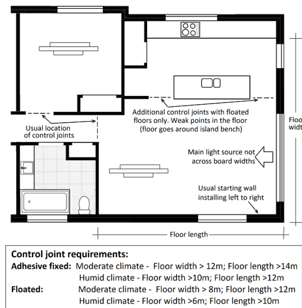
Figure 2 – Installation
